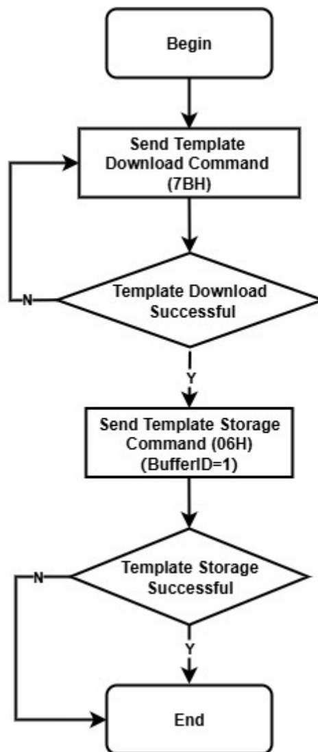
Function Example 8 : Speciadownload template process
