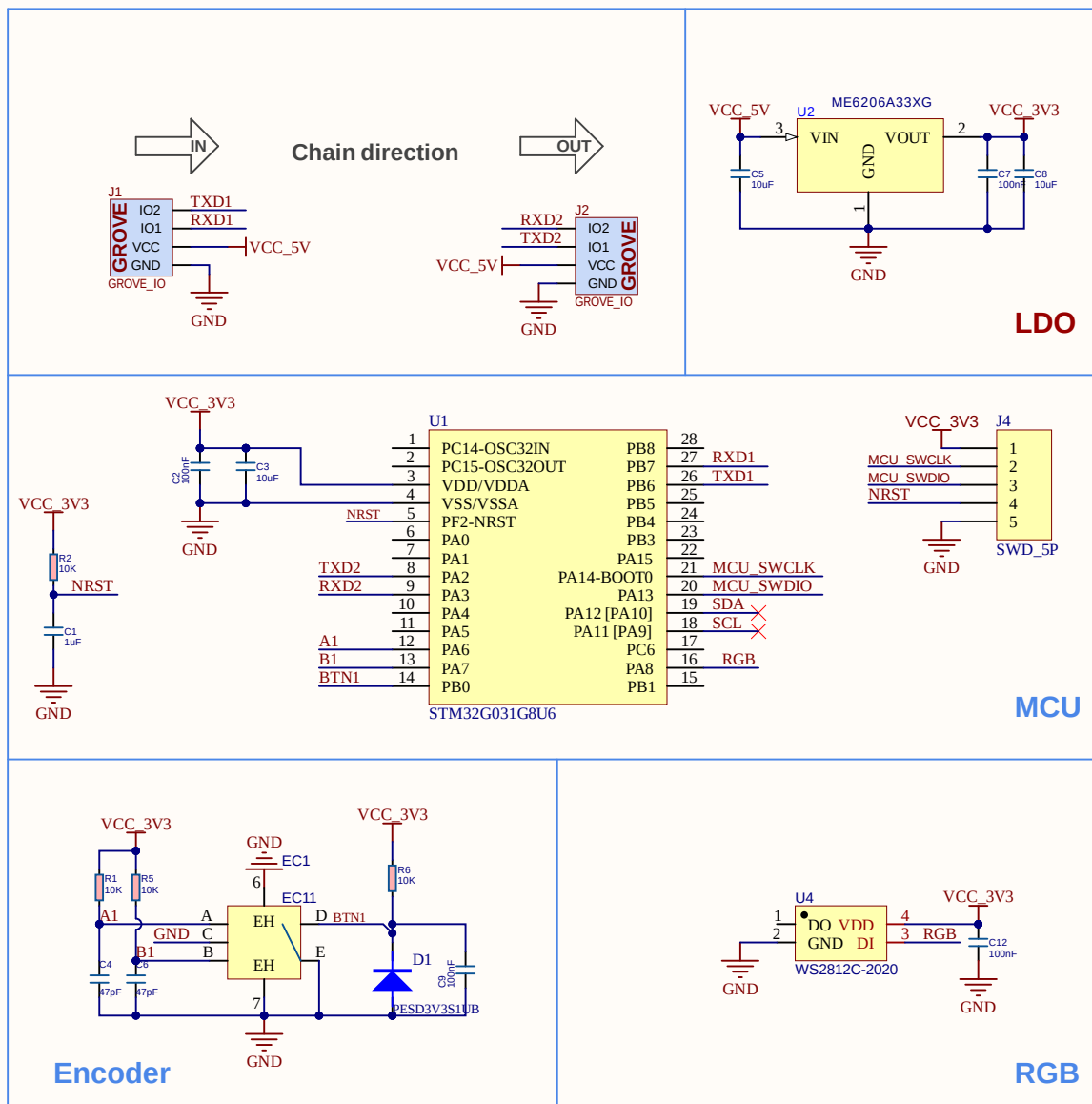
Chain Encoder
