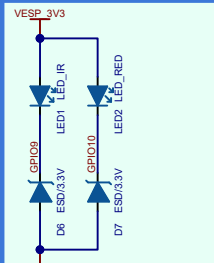
LED/IR
