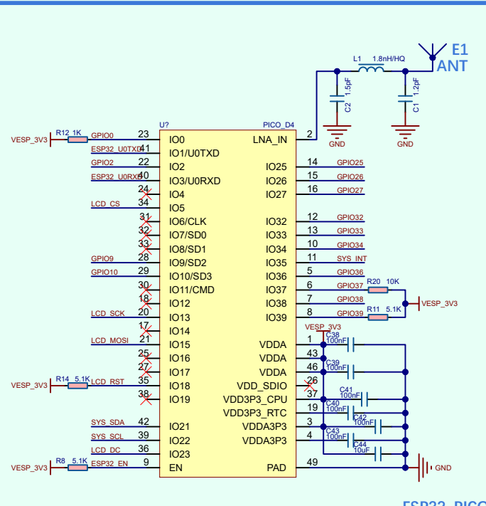
ESP32-PICO
