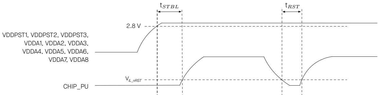
Figure 2-4. Visualization of Timing Parameters for Power-up and Reset
