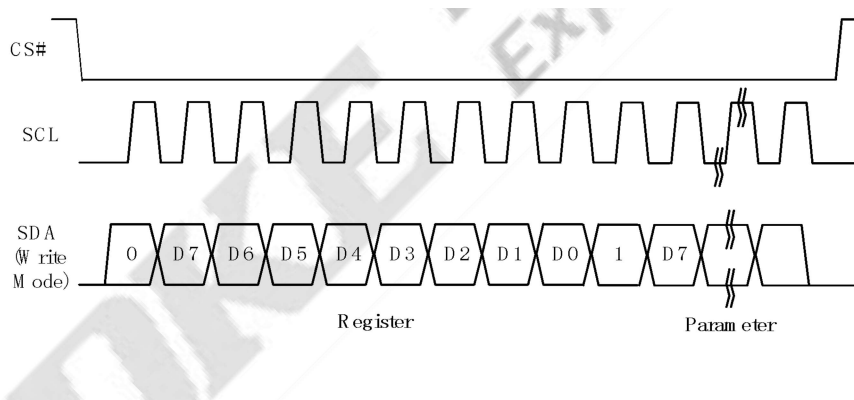
Figure 6-3: Write procedure in 3-wire SPI mode
