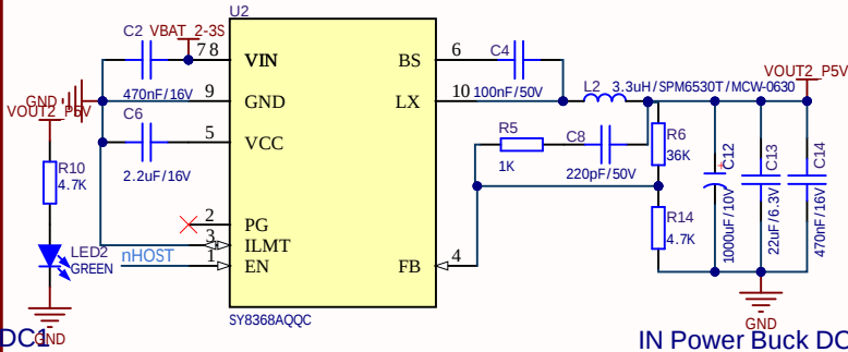
IN Power Buck DC-DC2
