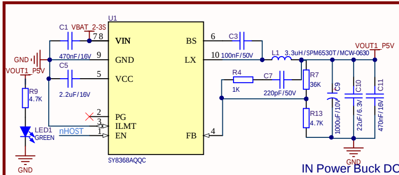
IN Power Buck DC-DC1
