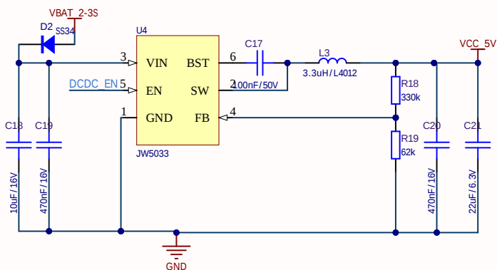
Sys Buck DC-DC
